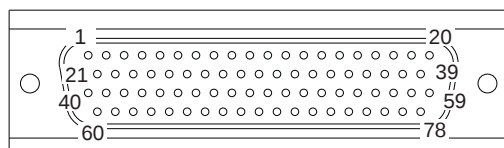
Figure 2: Model 3720-MTC-1.5 / 3.0 pin number identification
