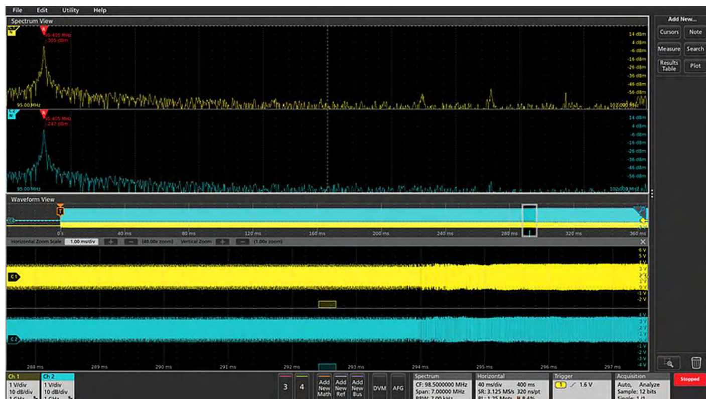
FIGURE 14. When debugging tasks demand it, multiple channels can be analyzed simultaneously. Here, two channels show the startup of a clock signal from two different points in a circuit.
