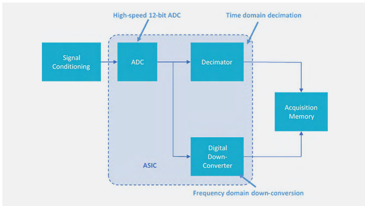
FIGURE 2. Digital down converters implemented on a custom ASIC enable simultaneous waveform and spectrum views with independent controls in the Tektronix 4, 5 and 6 Series MSOs.
