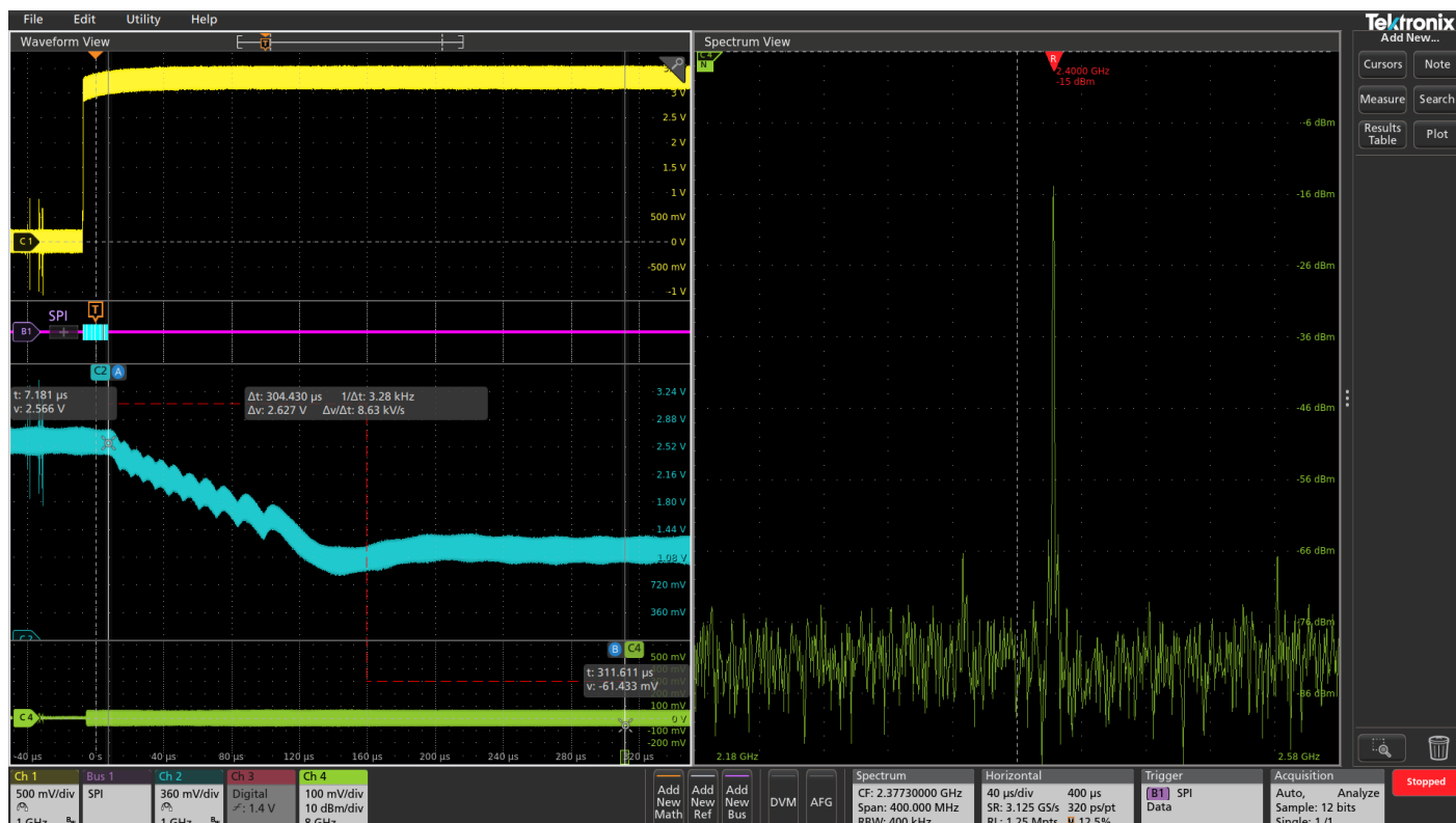
FIGURE 13. We are triggering on the SPI bus command that tells the VCO what frequency to tune to. In this case, it's 2.4 GHz. Using Spectrum Time, we were able to scroll through the acquisition and see when the RF output stabilized at 2.4 GHz. Then, using cursors, we can measure from the trigger event to Spectrum Time's location and see that it took 304 \mu s for the output to achieve the desired frequency.
