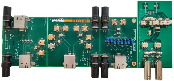
TF-XGbT test fixture
