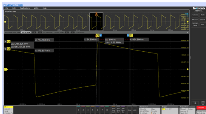
Droop measurement
