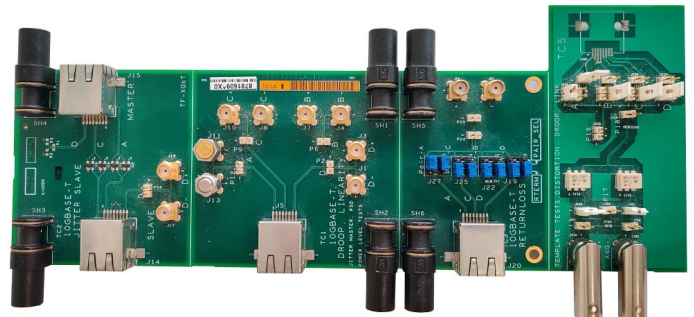
TF-XGbT test fixture
