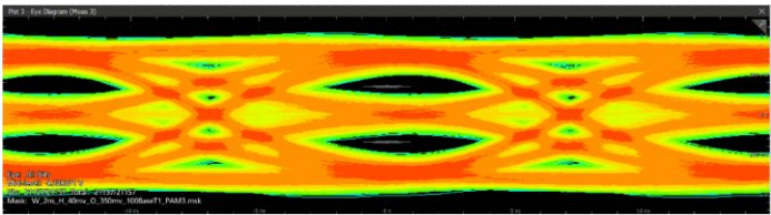
Automotive Ethernet Far End Eye diagram
