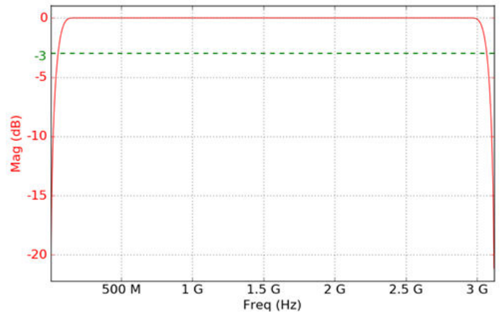
Hilbert response
