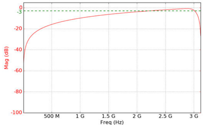
Differentiator response
