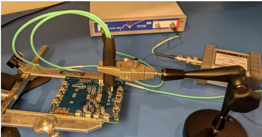
The Picotest P2102A probe performs the popular 2-port shunt-through impedance test. It may be hand-held or used with a probe holder.
