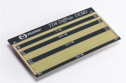
The Picotest P2103A demo board
