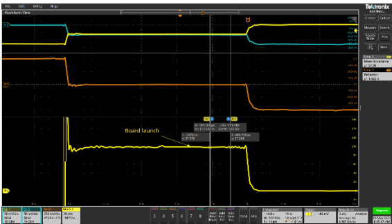
P2103A recorded differential signal, gamma function and 100 Ohm measurement
