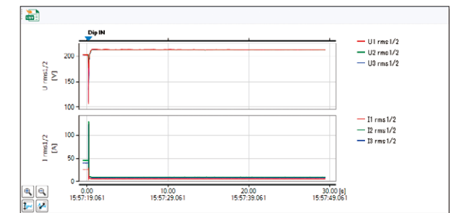
Example voltage dip screen (30 sec. event fluctuation data)
